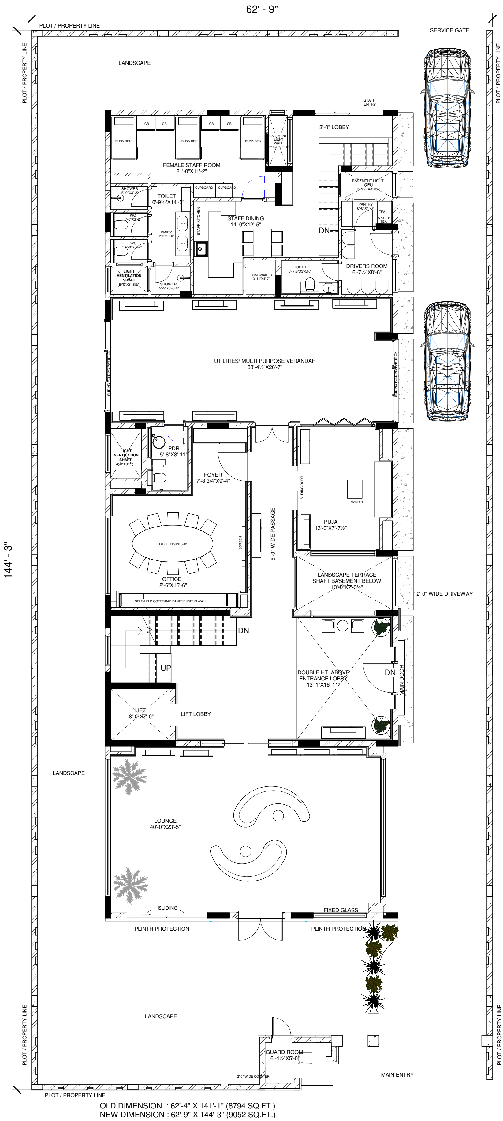
1 STILT FLOOR LAYOUT 1/8" = 1'-0"
